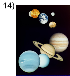
astronomy
