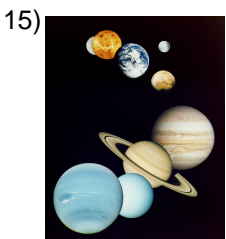
astronomy
